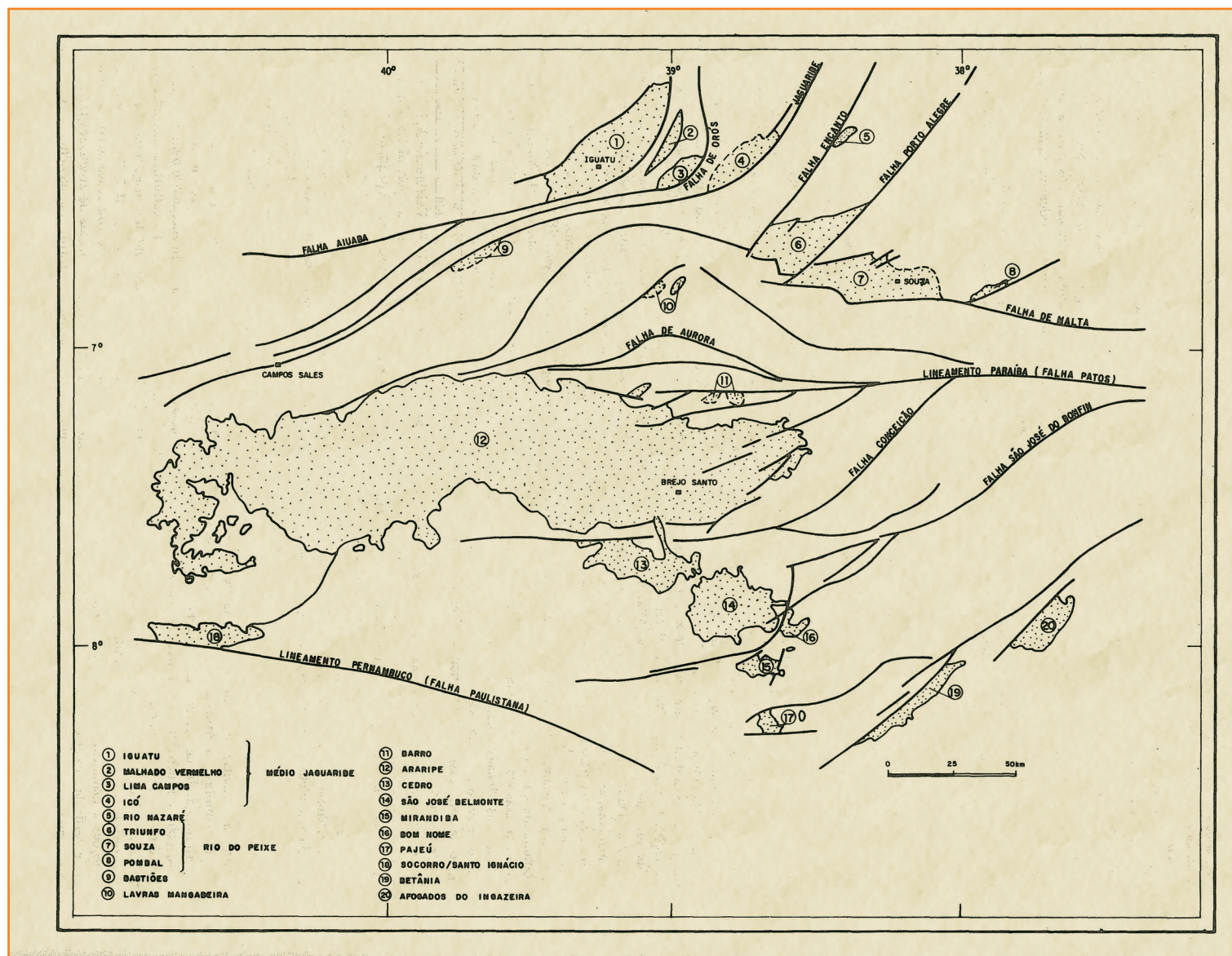
Figure 22 Schematic of the main polycyclic fault traces of the central Northeast part and associated sedimentary occurrences (Northeast Interior Basins).
