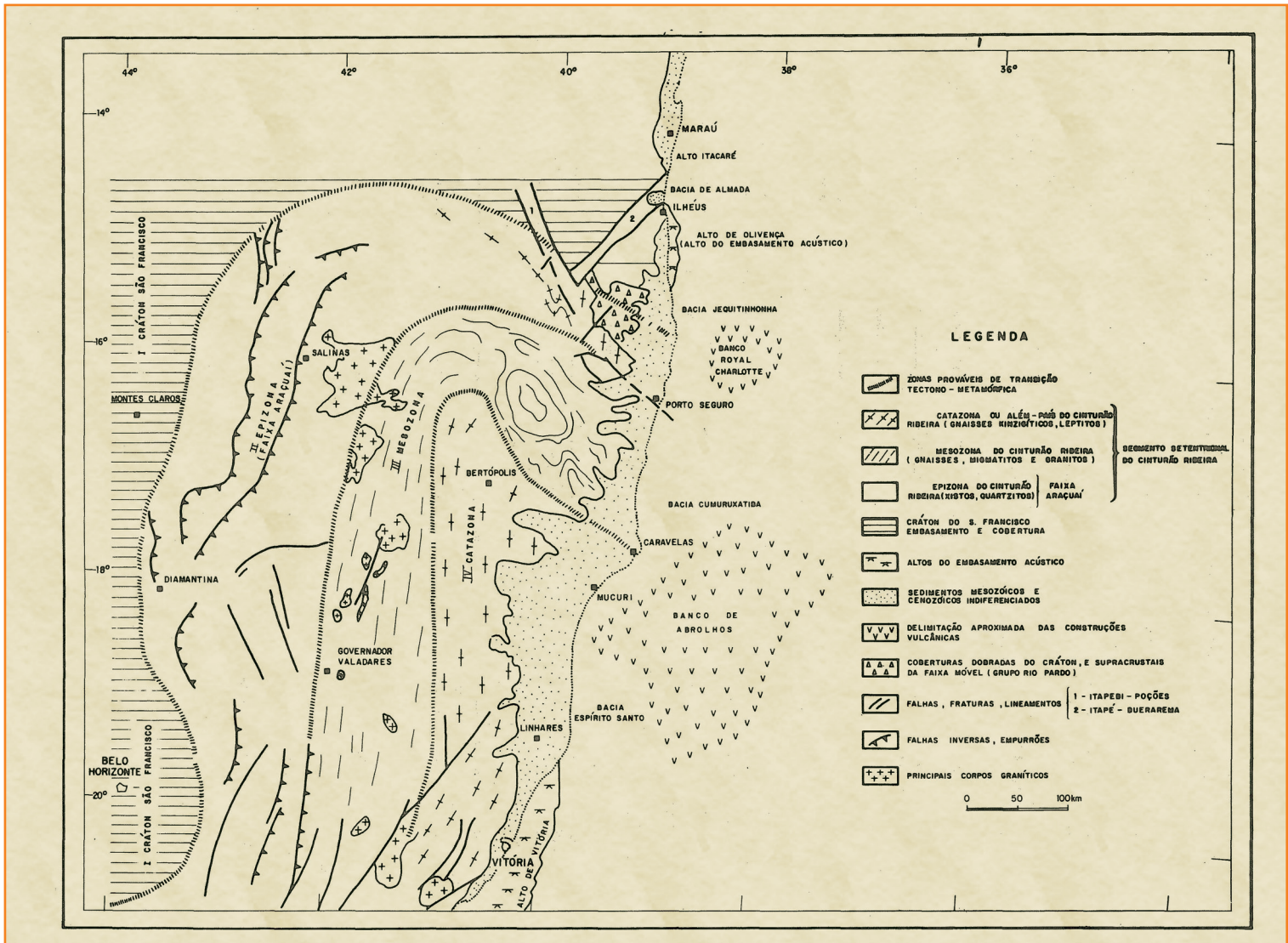
Figure 18 Schematic geological-geotectonic map of the basement of the Bahia-Sul and Espírito Santo Basins.
