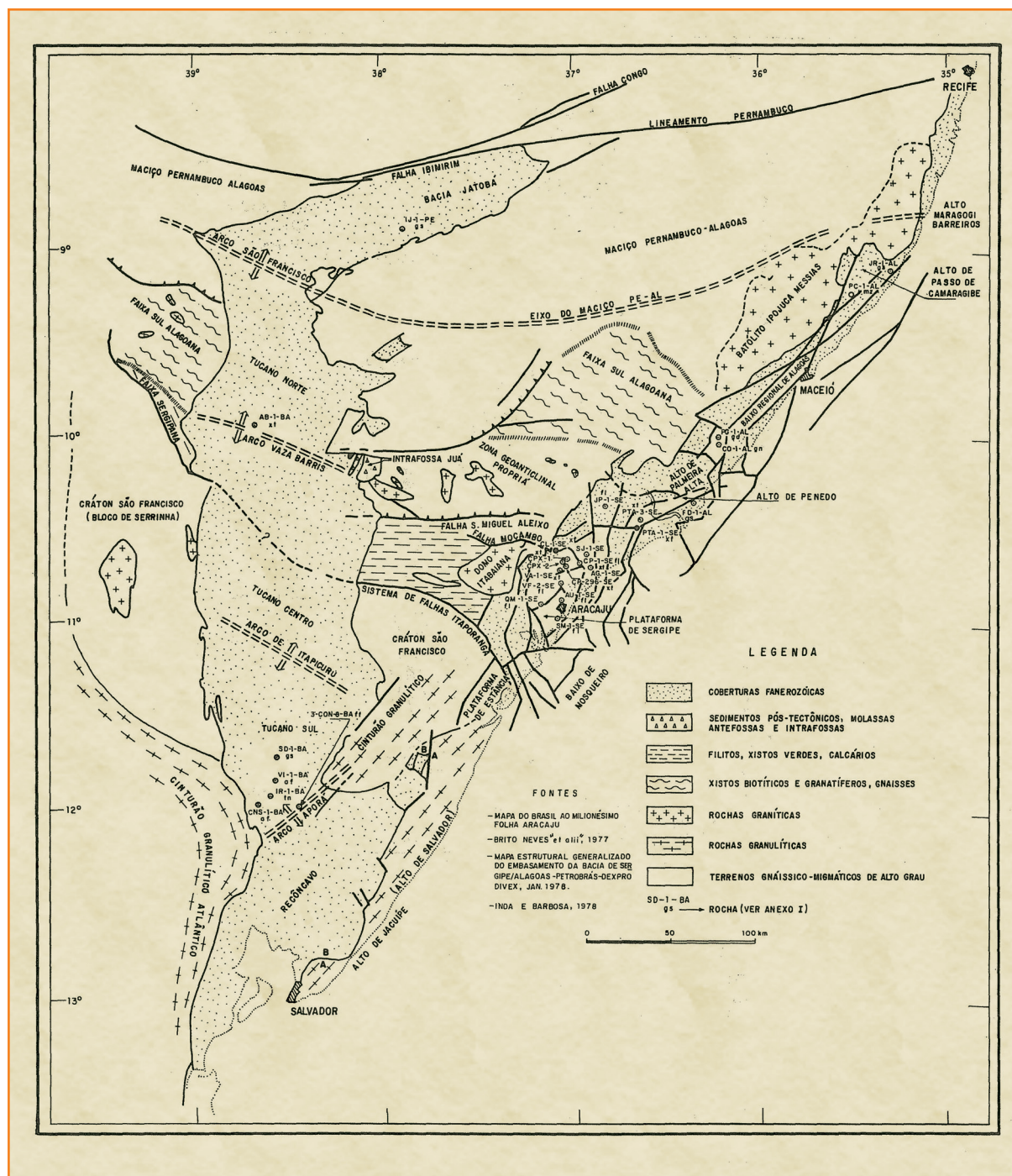
Figure 17 Schematic geological-geotectonic map of the Sergipe-Alagoas Basin basement.
