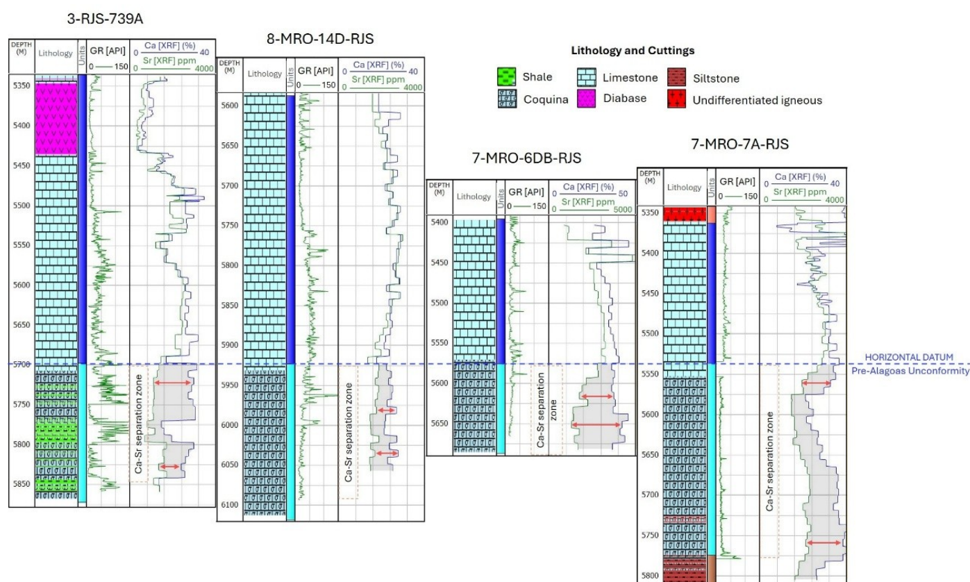
Figure 11. Four of the 12 well showing the Ca-Sr feature at the discordance between the Barra Velha and Itapema formations in the Mero Field.
